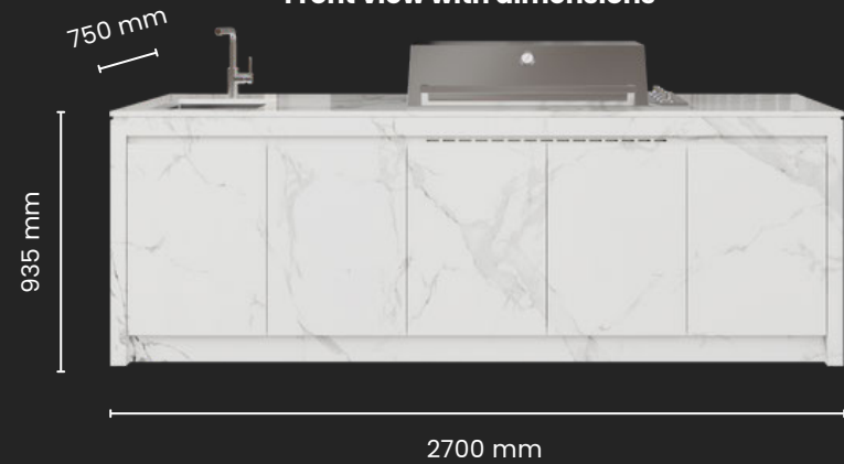
Front view with dimensions
